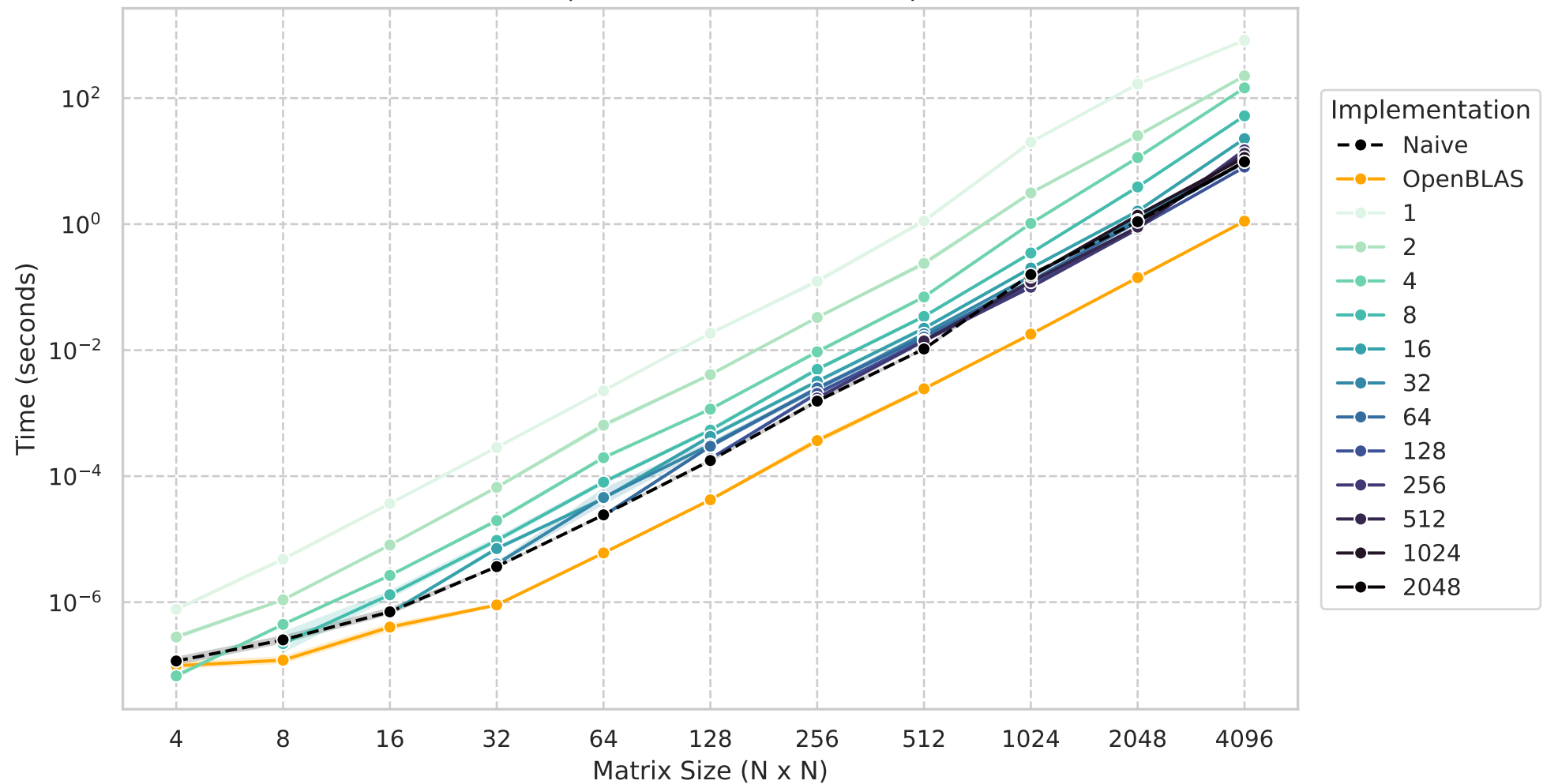
Matrix Multiplication Performance Comparison
