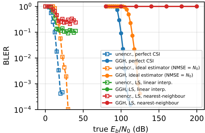
(a) UMi, n = 512
