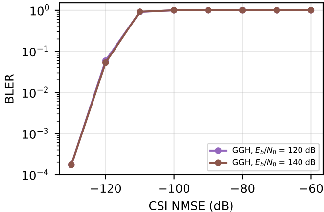
(b) required CSI accuracy
