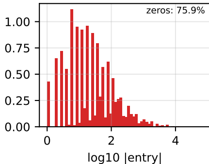
U: log10 |nonzero entries|
