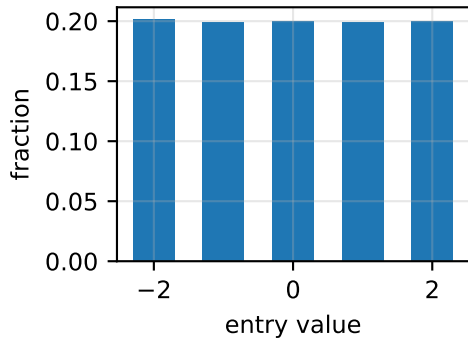
R off-diagonal (diag = 46)
