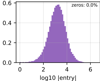
B: log10 |nonzero entries|
