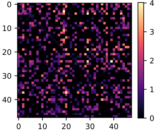
\log_{10} (1 + |U^{-1}|) (top-left 48 \times 48 )
