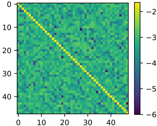
\log_{10} |R^{-1}| (top-left 48 \times 48 )
