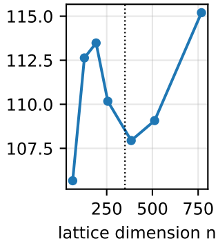
(c) dimension
