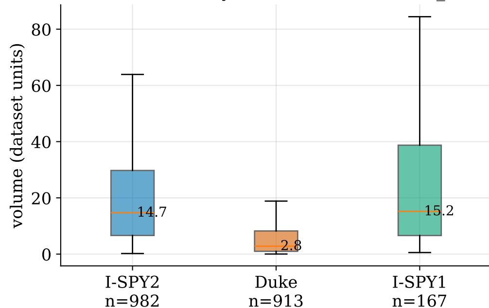
Tumour volume by cohort (metadata `tum_vol`)
