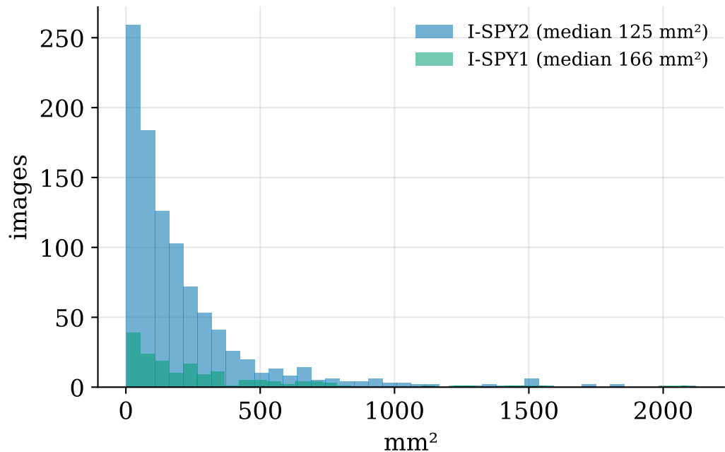
Tumour area on the saved slice
