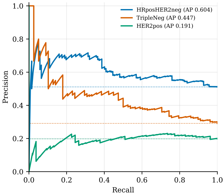
test03 — global test set dotted = class prevalence (chance)
