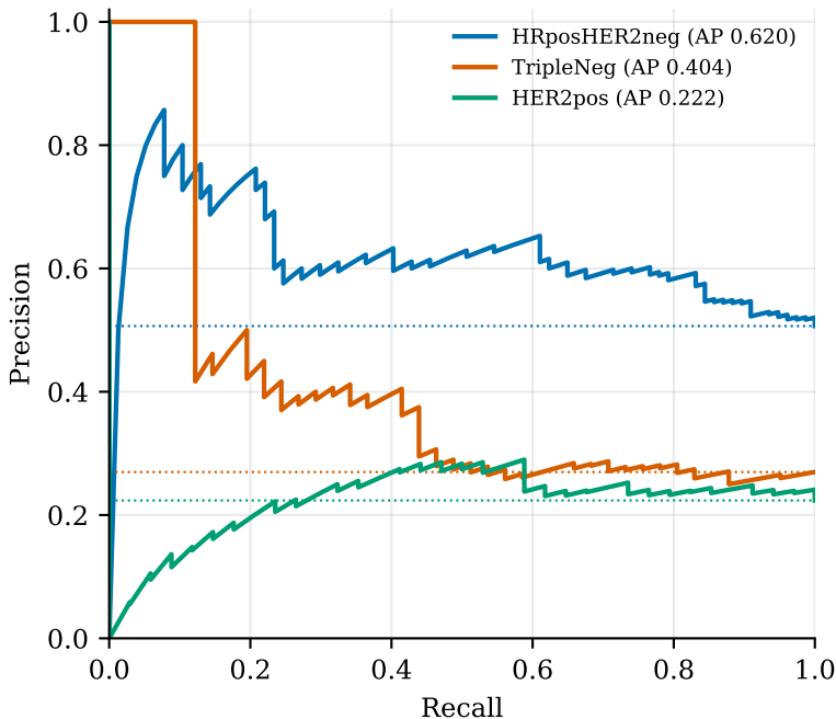
test03 — hospital_2 dotted = class prevalence (chance)
