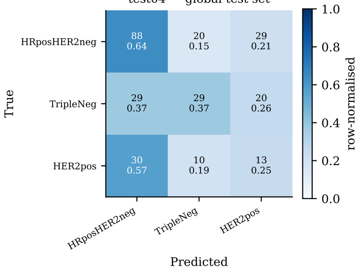
test04 — global test set
