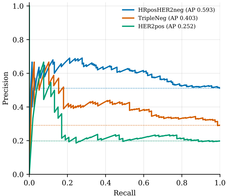
test05 — global test set dotted = class prevalence (chance)
