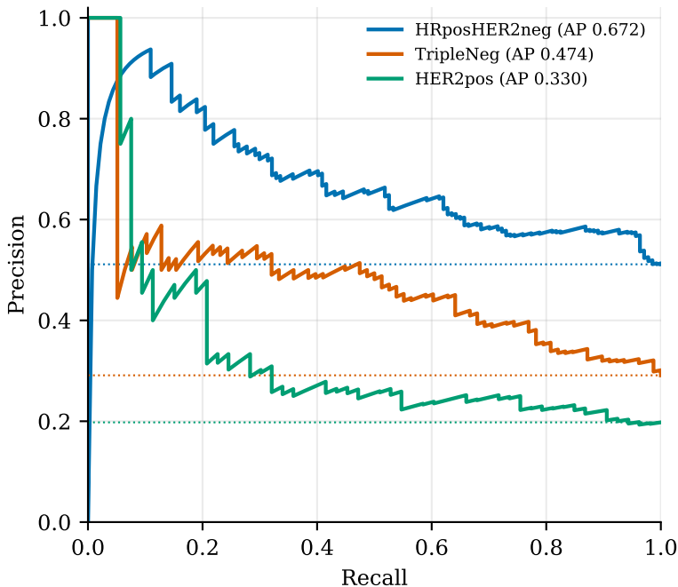
test06 — global test set dotted = class prevalence (chance)
