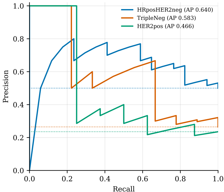
test09 — hospital_3 dotted = class prevalence (chance)
