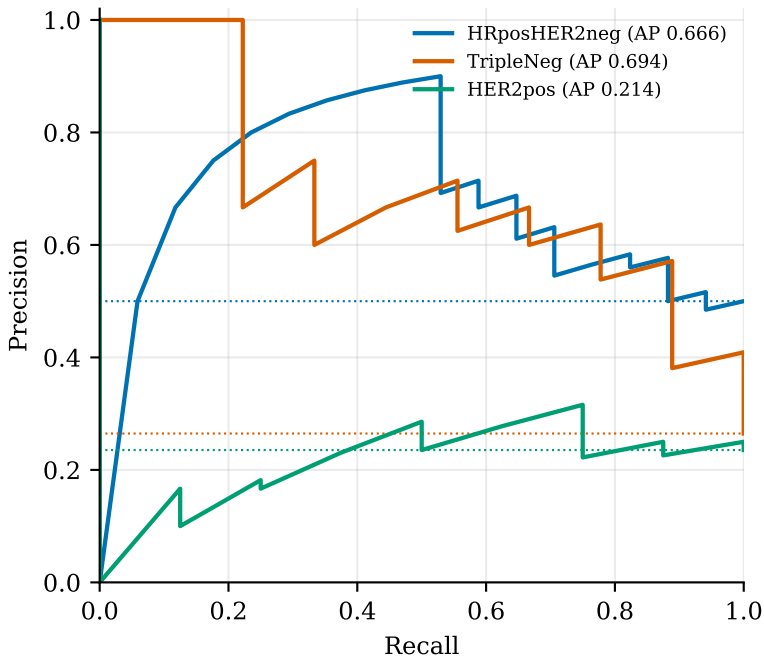
test09 — hospital_4 dotted = class prevalence (chance)
