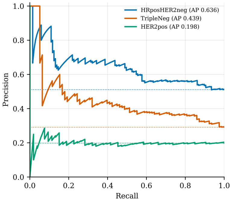
test13 — global test set dotted = class prevalence (chance)
