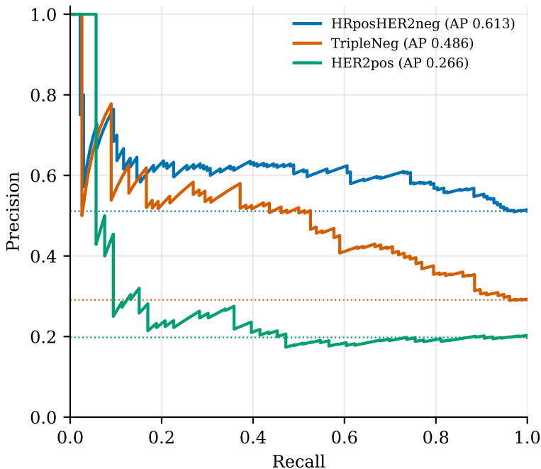
test01 — global test set dotted = class prevalence (chance)
