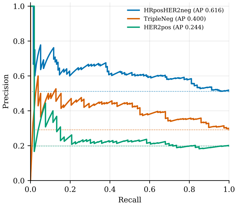
test04 — global test set dotted = class prevalence (chance)
