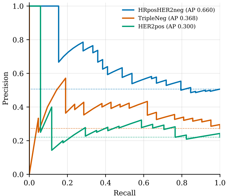
test06 — hospital_1 dotted = class prevalence (chance)
