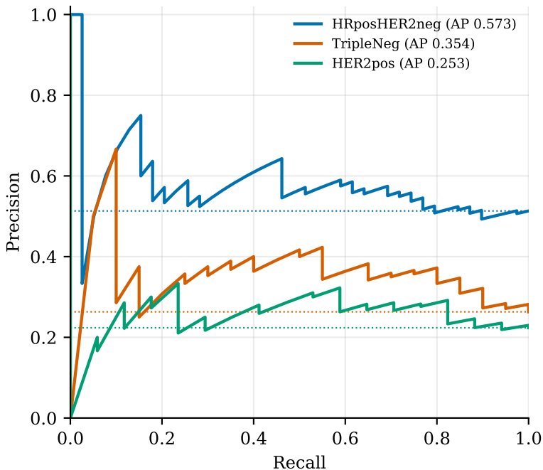
test06 — hospital_4 dotted = class prevalence (chance)
