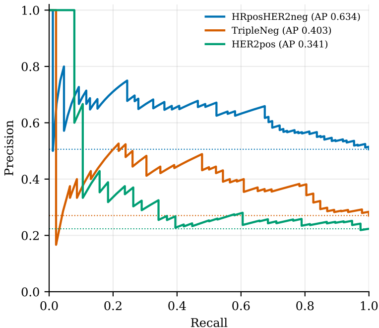
test09 — hospital_1 dotted = class prevalence (chance)
