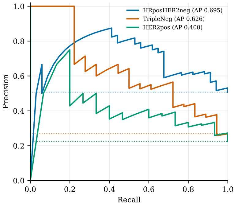
test09 — hospital_2 dotted = class prevalence (chance)
