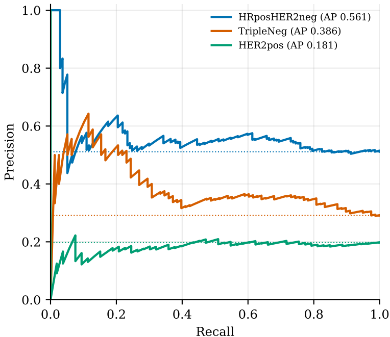
test10 — global test set dotted = class prevalence (chance)
