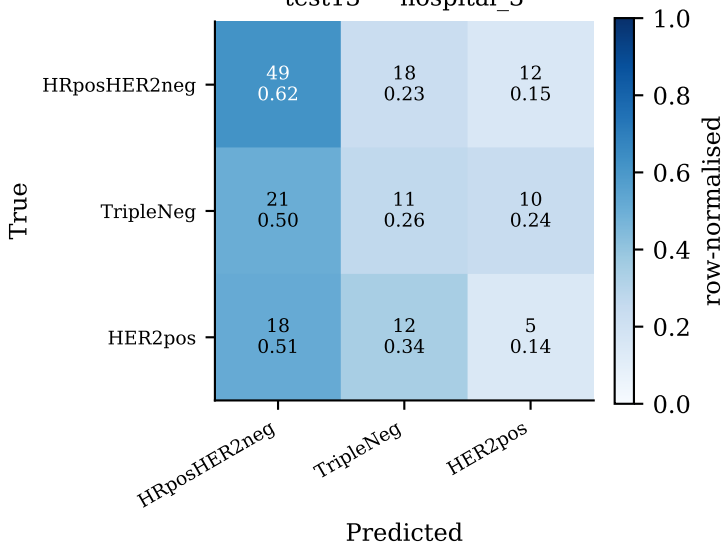
test13 — hospital_3
