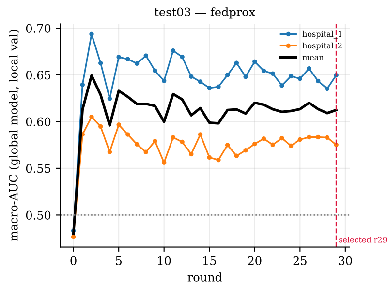
Federated round evolution — the arriving global model scored at each hospital
