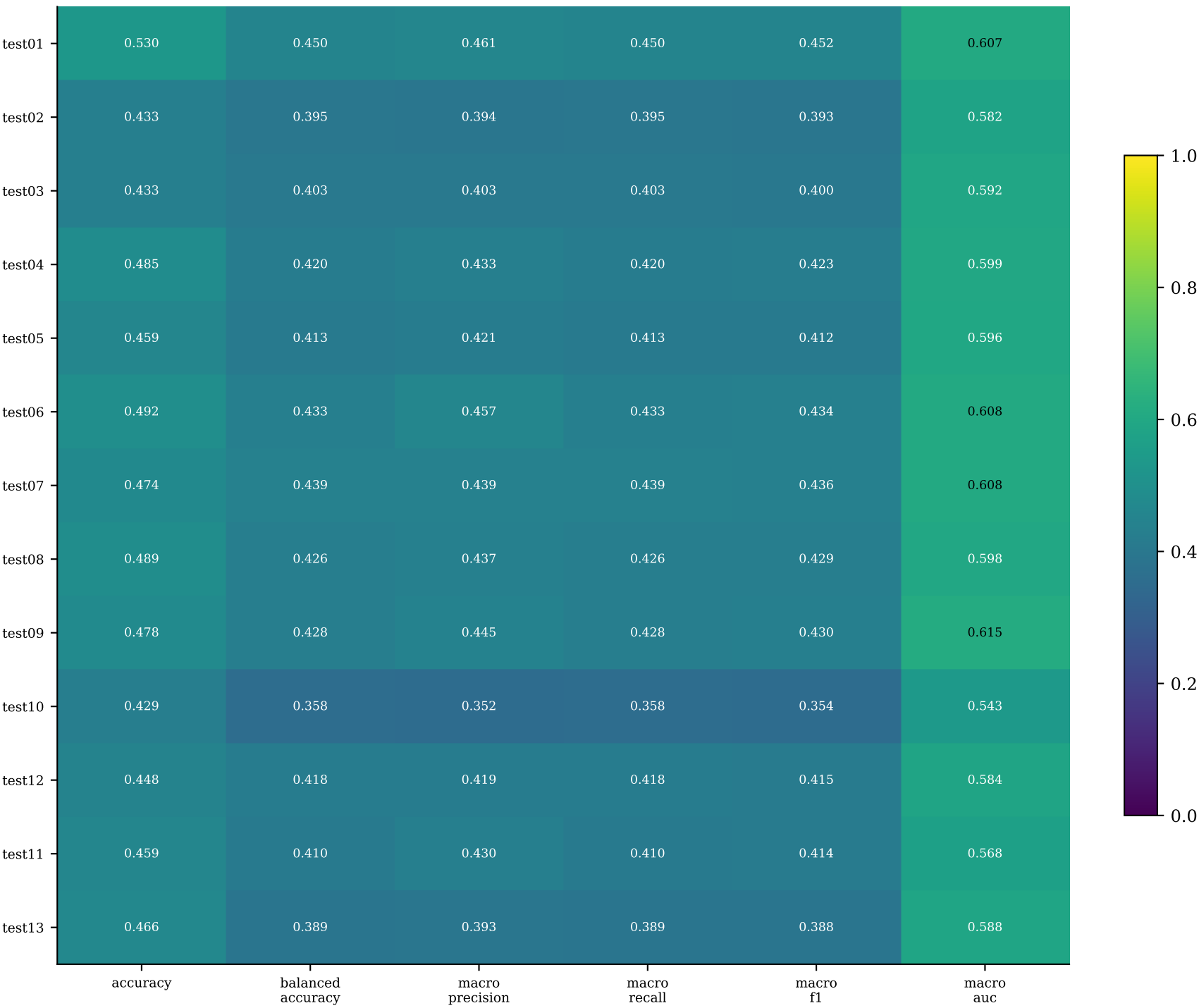
Metric comparison across all experiments
