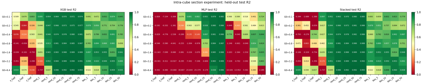
Figure 12. Within-cube sampling geometry: test R^2 per training geometry (columns) and cube (rows) for XGBoost (left), MLP (centre), and the stacked ensemble (right). Random coverage \geq 5-10 per cent reconstructs the held-out cells well in every cube; 50 per cent contiguous slabs fail in every cube; compact boxes are intermediate; 1 per cent random coverage is unstable, varying from R^2 \approx 0.9 to strongly negative between cubes.
