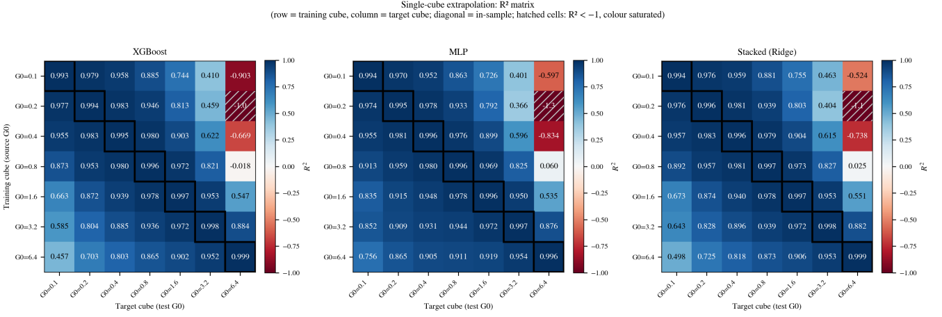
Figure 11. Single-cube transfer: log-space R^2 for models trained on one cube (rows) and evaluated on each cube (columns), for XGBoost (left), MLP (centre), and the stacked ensemble (right). Diagonal cells are in-sample fits. The colour scale is clipped to R^2 \in [-1, 1] ; hatched cells fall below -1 , with the actual value printed. Transfer quality decays with G_0 separation; values for separations of four or more geometric steps are poor and can be strongly negative.
