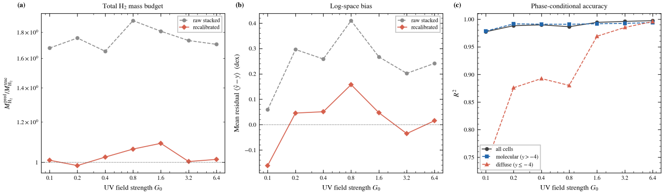
Figure 4. Mass budget and phase-conditional accuracy of the deployed (fully nested) pipeline of Section 5.5. (a) Total H 2 mass ratio per held-out fold: the raw stack (grey) over-predicts by \times 1.65 – 1.90 at every G_0 ; the mass-calibrated prediction (red) is within 9 per cent of the true mass in every fold. (b) Cell-mean log residual: the calibration also removes most of the mean bias. (c) Phase-conditional R^2 : molecular-phase accuracy is uniformly high ( R^2 \geq 0.98 ); the diffuse phase is hardest at low G_0 , where UV-exposed gas spans the steep transition.
