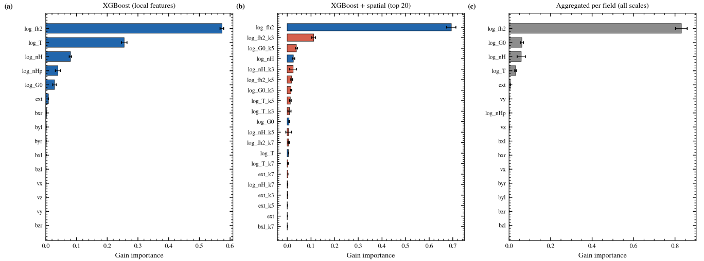
Figure 5. XGBoost gain importance, mean \pm std over the seven folds. (a) Pointwise model (15 local features): the solver-derived \log f_{\text{H}_2} dominates, followed by temperature and density. (b) Spatial-feature model, top 20 of 60 features (blue = local, red = neighbourhood means): f_{\text{H}_2} and its spatial averages fill the top ranks. (c) Importance aggregated per base field over all scales. Velocity and magnetic-field components are negligible in every view.
