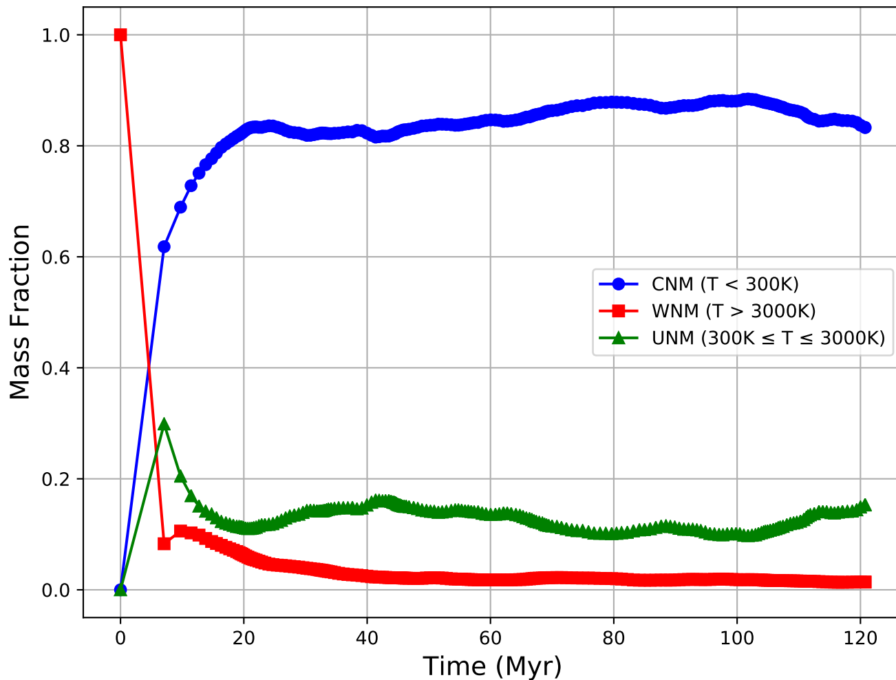
CNM, WNM, and UNM Mass Fractions Over Time
