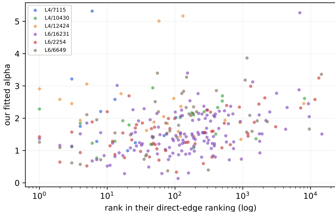
Amplification vs attribution rank
