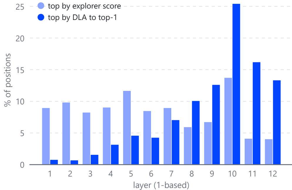
Layer of the top-ranked fired circuit
