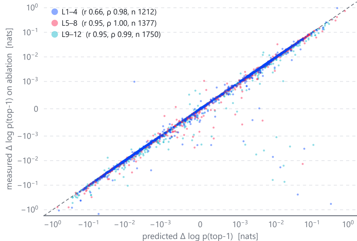
Attribution patching (total effect)
