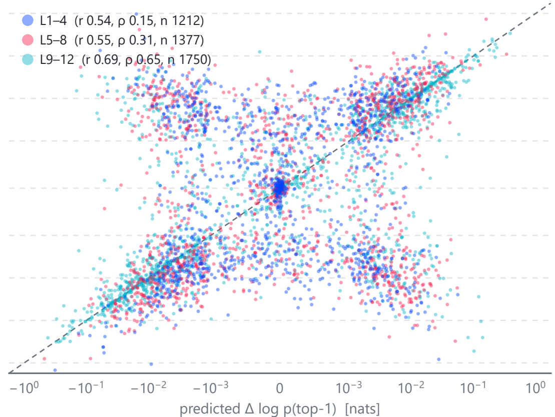
Direct logit attribution (064)
