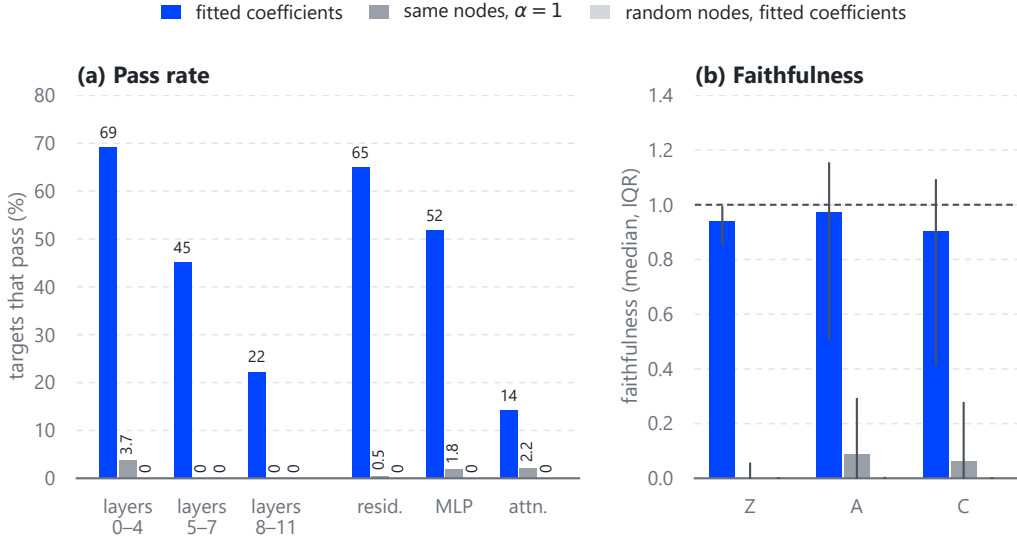
Figure 11: The coefficient triad on the production circuits. (a) The share of targets that pass the criterion of Section 4.4, by target depth band and site kind, for the circuits as fitted (blue; the full run, 14,994 circuits), the same nodes with every coefficient set to 1 (grey; 1,746 targets), and random nodes of the same size given the same coefficient fitting (light grey; 747 targets). (b) Median faithfulness under zero (Z), activating-mean (A), and contrast-mean (C) ablation, with interquartile ranges; 1 is perfect (dashed).
