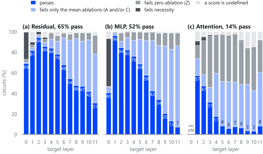
Figure 2: How the weighted circuits of 15,004 TuringLLM latents fare at the production sparsity penalty, by target layer and site kind. Each circuit is counted once: it passes the pre-stated criterion (faithfulness under Z, A, and C in [0.8, 1.5] and necessity \geq 0.9 , on held-out contexts); fails only the mean ablations (A, C, or both) while zero ablation and necessity hold; fails zero ablation while necessity holds; fails necessity; or has an undefined score (3%, counted as a fail). Numbers on the bars are pass rates (%), and panel titles give each site kind’s overall pass rate; layer-0 attention outputs have no upstream site.
