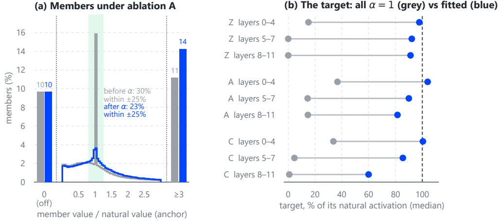
Figure 12: What the coefficients do to circuit members (600 production circuits). (a) Each member’s value in the circuit-only run divided by its value in the unmodified model, at the target’s anchors on held-out contexts, under activating-mean ablation, before (grey) and after (blue) its coefficient; members active in the unmodified model, pooled over circuits. The bars at either side collect members that left their site’s Top-K (“0, off”) and members at three or more times their natural value; both groups are mostly members that fire weakly in the unmodified model, and together they carry \sim 8\% of the circuits’ contribution to their targets. (b) The target’s activation in the circuit-only run as a share of its natural activation, median over circuits, with every coefficient set to 1 (grey) and with the fitted coefficients (blue), by ablation method and target depth band.
