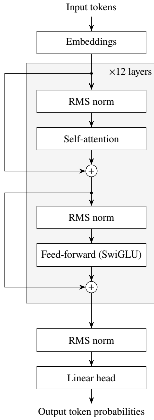
Figure 5: TuringLLM-1.0-254M architecture: a 12-layer pre-norm decoder-only transformer with RMSNorm and a SwiGLU feed-forward block. The circuit-discovery pipeline attaches SAEs at three sites per layer: attention output, MLP output, and the residual stream.
