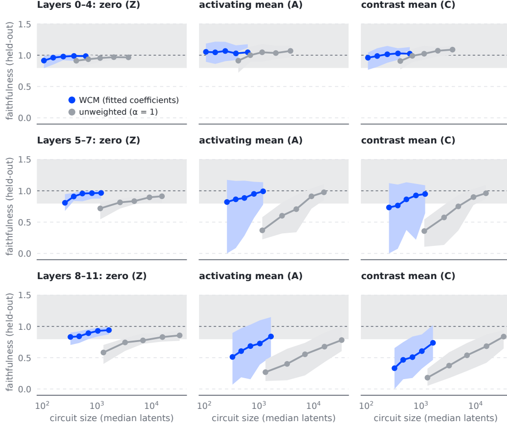
Figure 15: Weighted against unweighted circuit masking by ablation method (rows: target depth band; columns: zero ablation, and mean ablation over activating and over contrast contexts). Median held-out faithfulness and interquartile range against median circuit size, one point per sparsity penalty; the grey band is the pass band [0.8, 1.5] . The gap between the methods is smallest under zero ablation, largest under the two mean ablations, and widens with depth.
