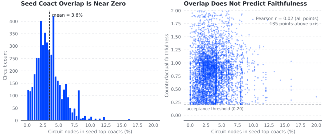
Figure 21: Discovered dependencies are not co-activation neighbourhoods (Appendix F). Left: distribution of the percentage of each circuit’s nodes that appear among its target’s top co-activation partners (mean 3.6%). Right: the same overlap against the circuit’s sufficiency to induce (Pearson r = 0.02 over all points; 135 of 4,741 points lie above the truncated axis). The dashed line marks the acceptance threshold (0.20), the minimum sufficiency to induce an accepted circuit can have. Statistics are over the 4,741 circuits with post-analysis co-activation metrics from the 7,525-circuit run.
