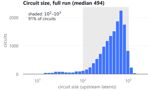
Figure 16: Circuit sizes in the production run at the production sparsity penalty: 91% of circuits hold 10^2 – 10^3 upstream latents (shaded); median 494.
