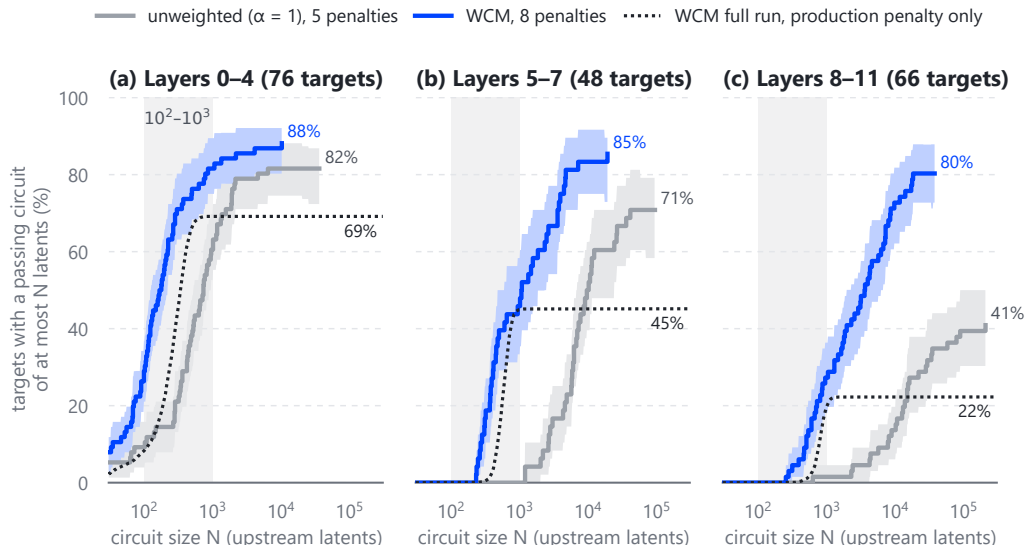
Figure 3: Fitted coefficients explain more targets at every circuit budget. For each target depth band, the share of 190 sweep targets with a circuit of at most N upstream latents that passes the criterion of Section 4.4 (faithfulness under Z, A, and C in [0.8, 1.5] and necessity \geq 0.9 , on held-out contexts), taking each target’s smallest passing circuit over the sparsity penalties it was fitted at: weighted circuit masking (blue) at eight penalties, \lambda from 4 \times 10^{-3} to 2.5 \times 10^{-5} , and unweighted circuit masking ( \alpha = 1 , grey) at five, 10^{-3} to 10^{-5} . Targets that never pass count as unexplained; shading is a 90% bootstrap interval over targets, and each curve ends at the largest circuit fitted. Dotted: the full run ( \sim 15,000 targets) at the production penalty alone, which levels off at that penalty’s pass rate.
