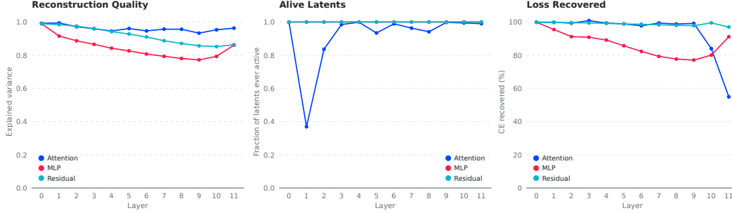
Figure 7: Quality of the 36-SAE bank by site. Left: explained variance of each SAE’s reconstruction. Middle: fraction of latents that fired at least once over the full collection pass. Right: percentage of the cross-entropy gap recovered when splicing each SAE’s reconstruction into the model, relative to zero-ablating the site.
