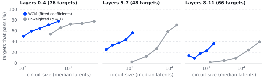
Figure 13: The pass-rate frontier for every target depth band: the share of targets that pass the criterion of Section 4.4 against median circuit size, one point per sparsity penalty, for weighted circuit masking (blue) and unweighted circuit masking ( \alpha = 1 , grey). 190 targets, protocol v1.
