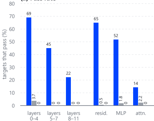
(a) Pass rate
