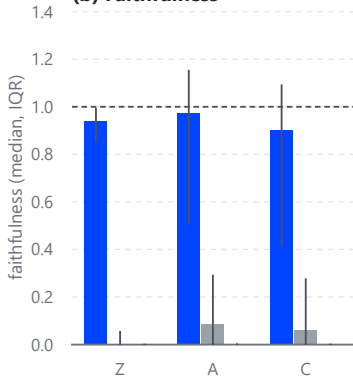
(b) Faithfulness
