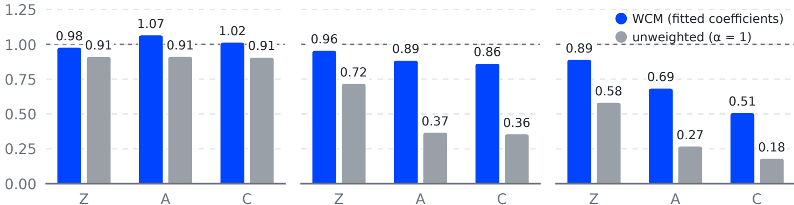
Layers 0-4 (76 targets) 238 vs 413 latents
