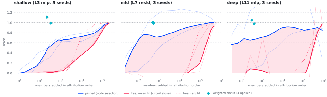
Figure 2: Control is sparse; faithfulness is collective; amplitudes collapse its cost. Cumulative score against members added in attribution order (three seeds per depth band: median curves, individual seeds ghosted; position-aware path attribution, percentile selection). Pinned faithfulness (node selection) rises steeply within 10^2 – 10^3 members, while free faithfulness (the circuit alone, at natural amplitudes) sits near zero until 10^4 – 10^5 members, under the mean fill (solid) and zero fill (dashed), each free variant naming its semantics. The shaded pinned–free gap widens with seed depth. Diamonds: weighted circuits discovered on the same seeds (Section 5.2), scored with their learned amplitudes applied under the zero fill, a few hundred members reaching the score the natural-amplitude curve needs 10^5 for.
