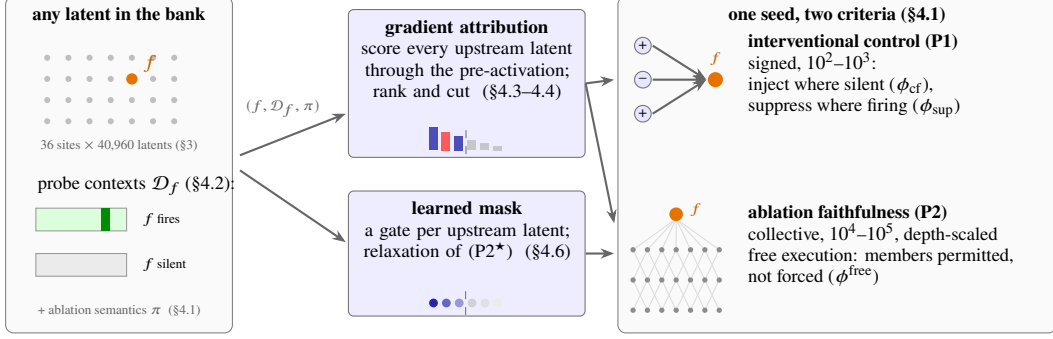
Figure 1: Overview. For any SAE latent f , with no behavioural task, a per-seed problem instance (f, \mathcal{D}_f, \pi) is formed from stored contexts where the seed fires and retrieved contexts where it is silent (§4.1). Discovery runs by gradient attribution (counterfactual and ablation objectives, ranked and cut) and by learned-mask optimisation (a gate per upstream latent). The discovered circuit is examined under two distinct criteria: interventional control (P1), validated by intervening on the seed itself, and ablation faithfulness (P2), the measured cost of the circuit reproducing the seed alone under free execution, spanning every upstream site. Control is concentrated; faithfulness is collective, position-local, and depth-scaled (§5.1).
