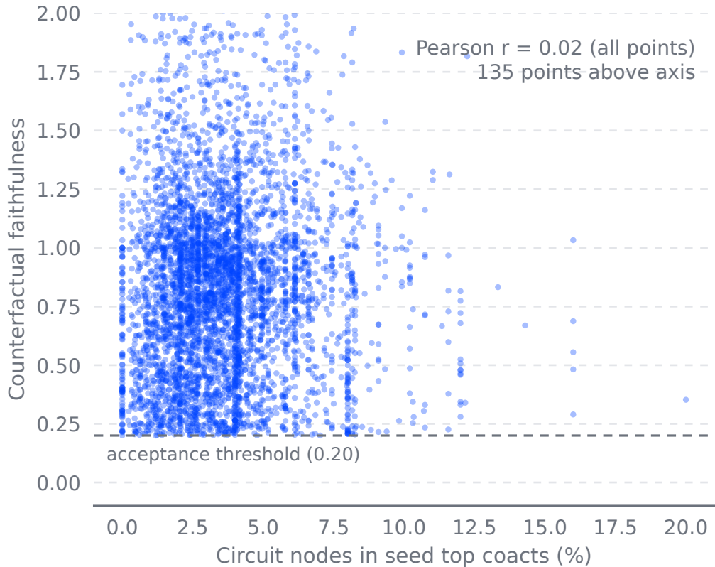
Overlap Does Not Predict Faithfulness
