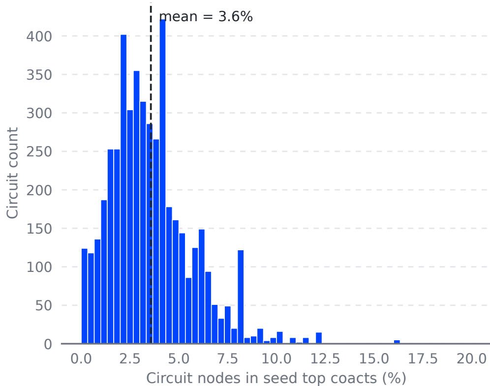
Seed Coact Overlap Is Near Zero
