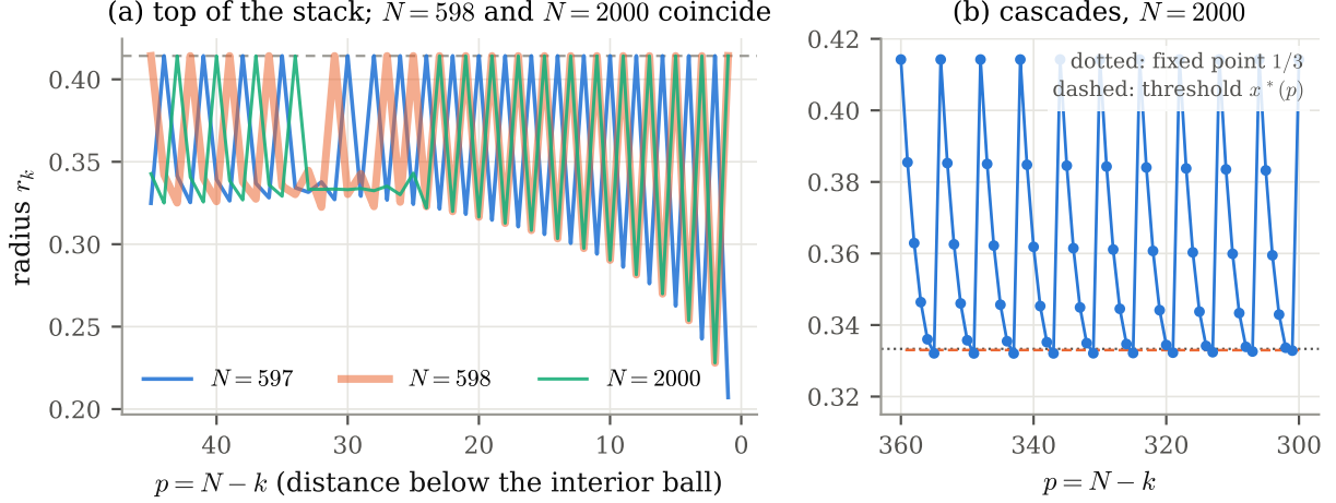
Figure 3: (a) The top 45 layers for N = 597, 598 and 2000 , plotted against p = N - k . Layers alternate between the cap and a radius pinned by the layer below. For N = 597 the top face layer ( p = 1 ) is pinned, giving r_N = \sqrt{2} - 1 ; for N = 598 and N = 2000 it is capped, giving 3 - 2\sqrt{2} , and these two curves are identical over the whole window. (b) Cascades deep in the stack for N = 2000 : each run descends towards the fixed point 1/3 and resets to the cap once a radius falls below the threshold x^*(p) .
