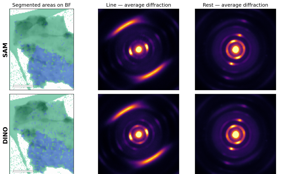
Column 1: Line (blue) and rest (green) areas overlaid on the virtual bright-field; vacuum = grayscale; scale bar 500 nm (16 nm/px). Columns 2-3: average diffraction of each region (log, central 260 px). Line domains: IoU = 0.74, Dice = 0.85, containment(SAM in DINO) = 0.85. Beam-masked Pearson r of average patterns: SAM_line vs DINO_line = 0.999; SAM_rest vs DINO_rest = 0.999; Line vs rest = 0.48-0.54 (incl. cross terms) – the two methods isolate the same, diffraction-distinct, oriented domain.
