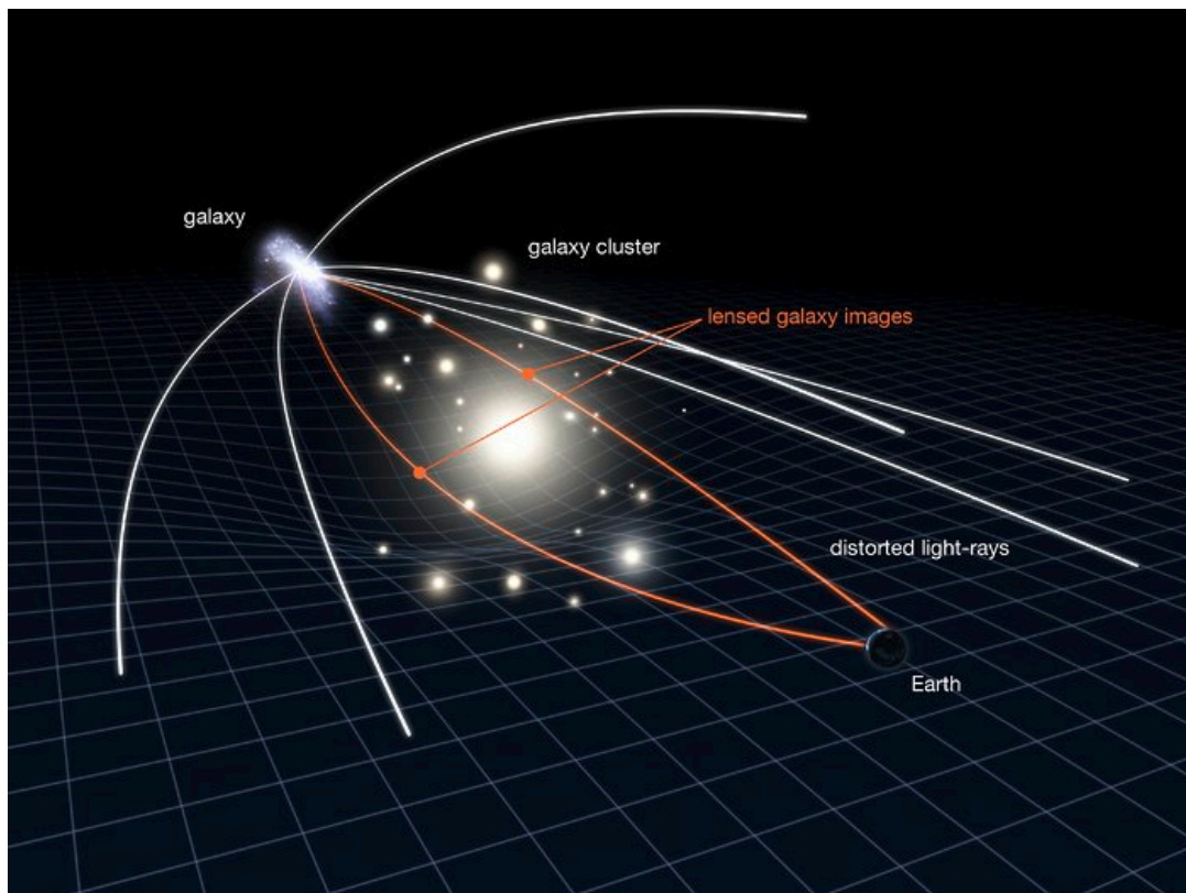
Figure 11: 来源: https://esahubble.org/images/heic1106c/
