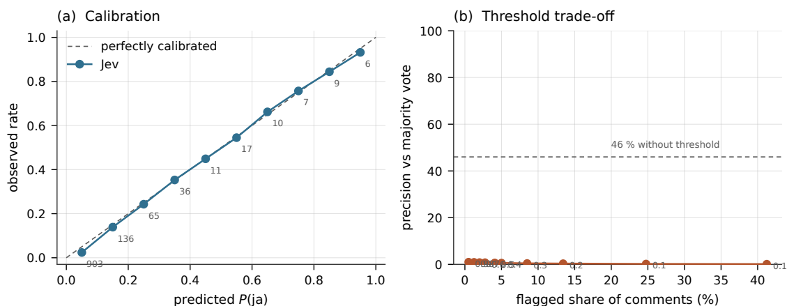
Figure 11. (a) Jev’s P(ja) against the four-model majority vote: observed reactant rate per probability bin versus the predicted probability (grey = the diagonal). This is alignment with a consensus proxy, not calibration against human labels. (b) The precision – coverage trade-off as the threshold t on P(ja) rises; the 46% line is Jev’s threshold-free precision.
