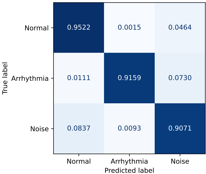
C. Global OOF Confusion Matrix
