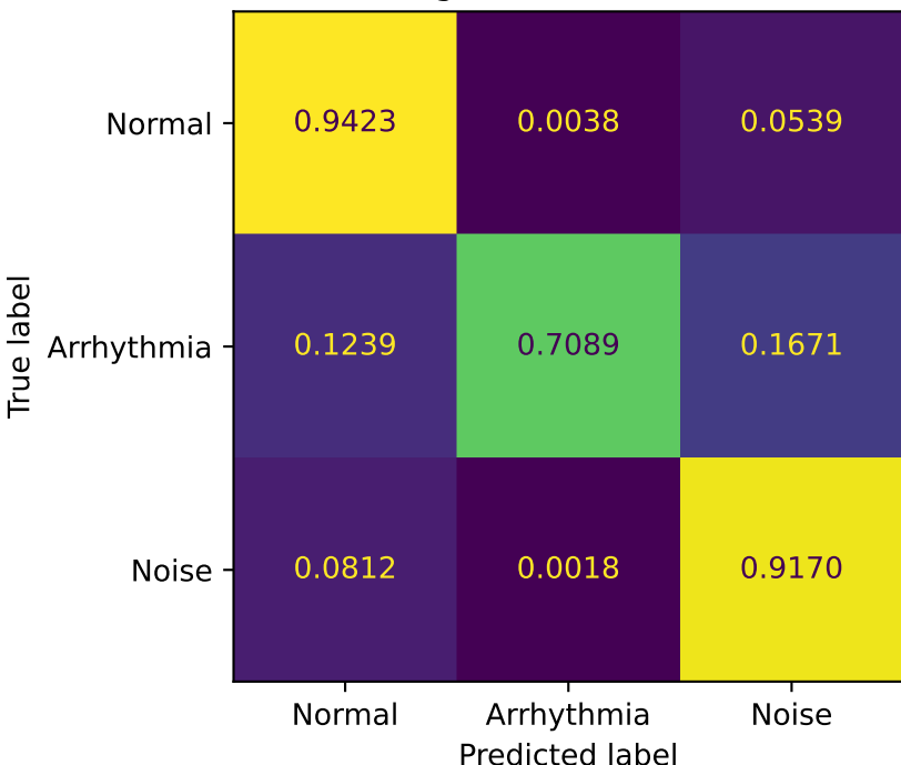
E. External Test Confusion Matrix Weighted F1 = 0.9306
