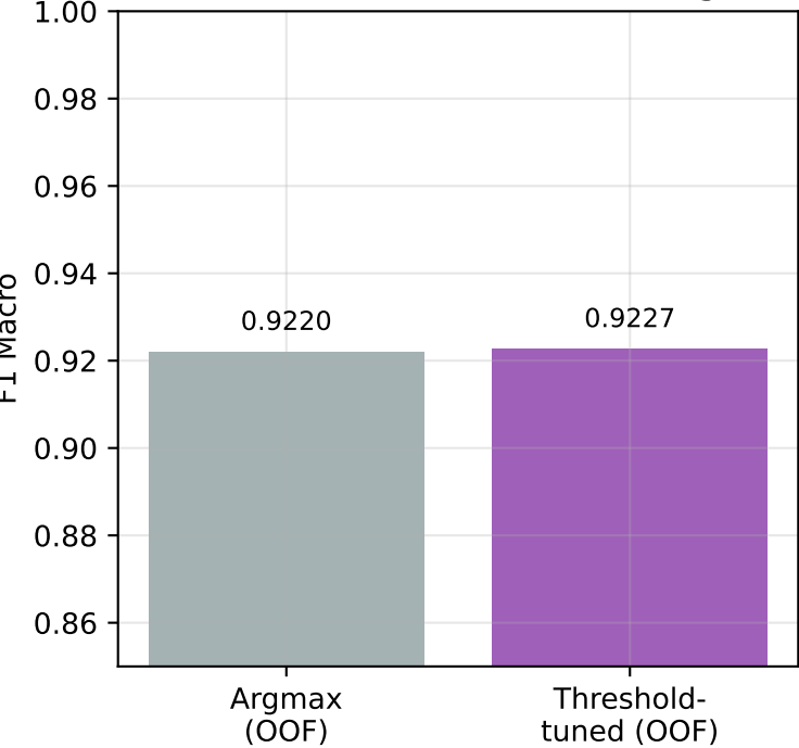
D. Effect of Threshold Tuning
