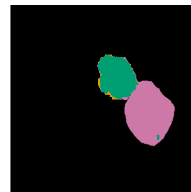
Pixel errors
