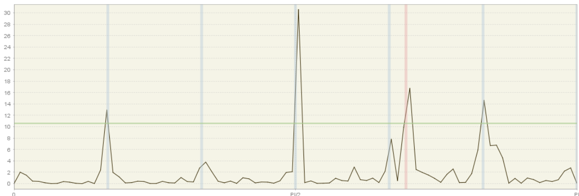
Figure 258: Periodogram with seasonal (grey) and calendar (red) frequencies highlighted
