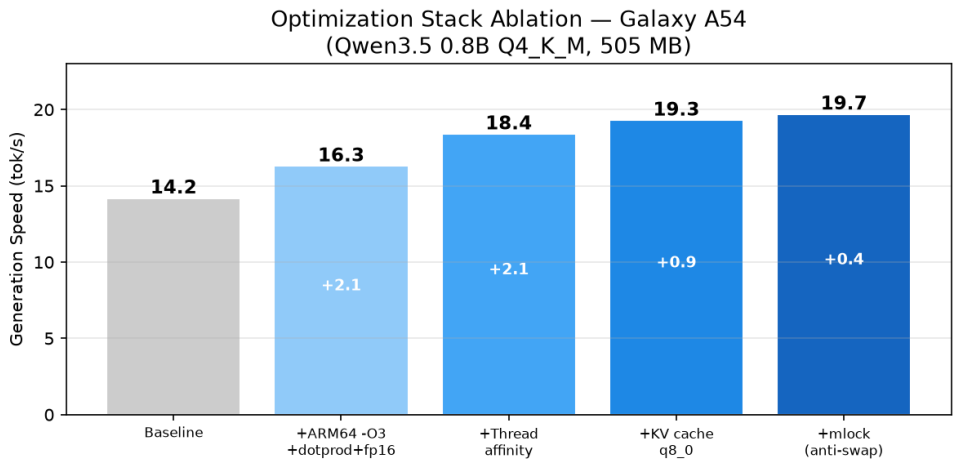
Figure 2. Additive contribution of each optimization step on Galaxy A54. The complete stack yields a 39% improvement over baseline.
