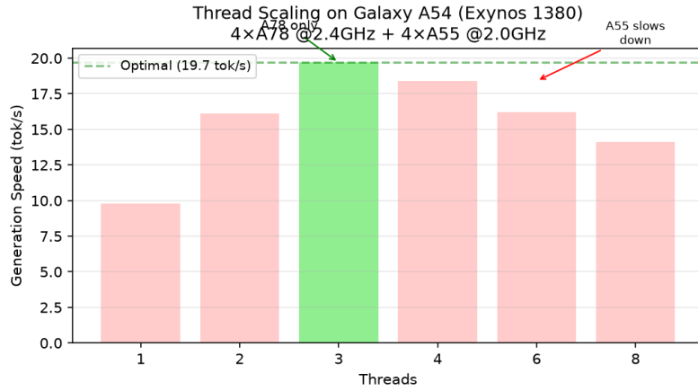
Figure 3. Thread scaling on Galaxy A54. Optimal performance at 3 threads (A78 cores only); adding A55 cores degrades throughput due to their \sim 3\times lower per-core bandwidth.
