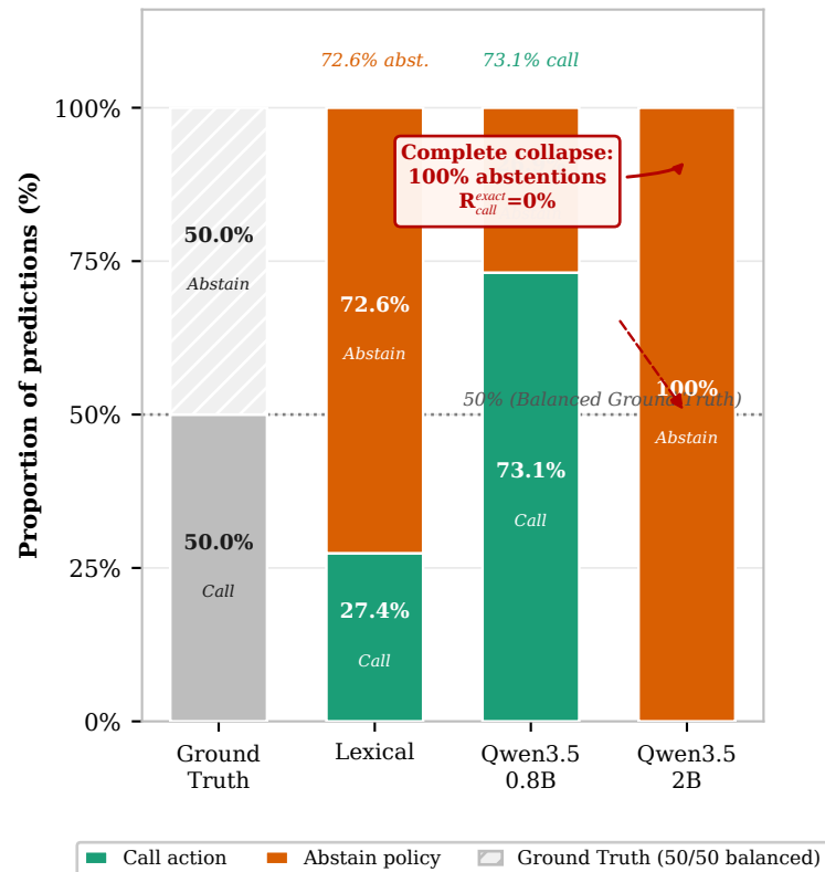
B — Predicted Action (Call vs. Abstain) vs. Ground Truth (Phrase-Disjoint Test)
