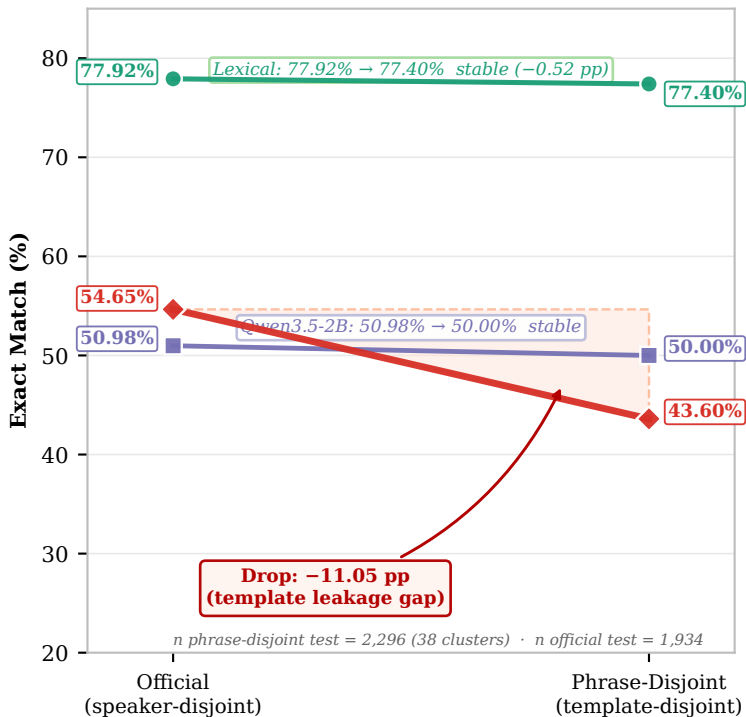
A — Template Leakage: Official vs. Phrase-Disjoint (Exact Match %)
