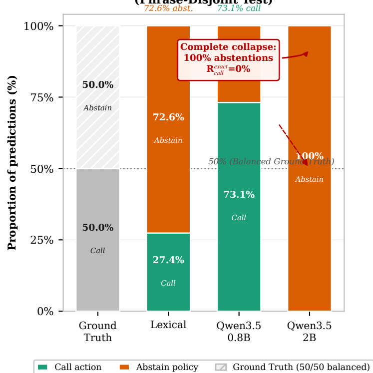
B — Predicted Action (Call vs. Abstain) vs. Ground Truth (Phrase-Disjoint Test)
