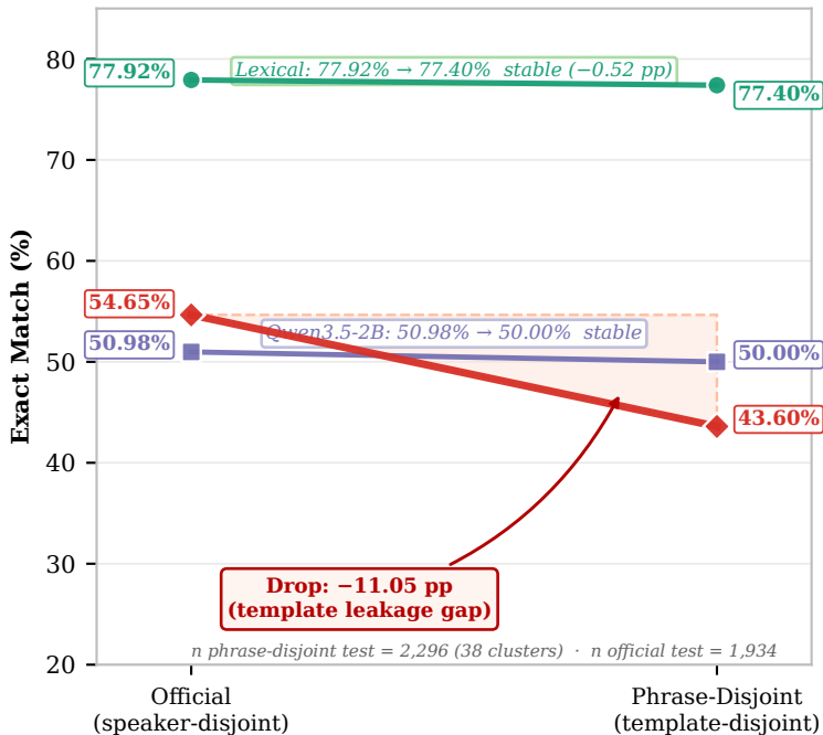
A — Template Leakage: Official vs. Phrase-Disjoint (Exact Match %)
