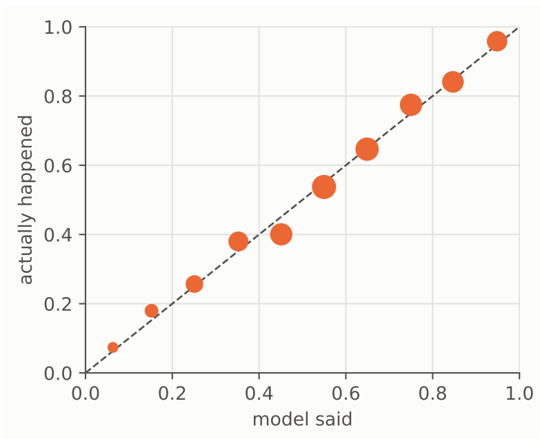
Figure 11.1: Win-chance calibration, 2021–2025: what the model said vs how often it happened.
