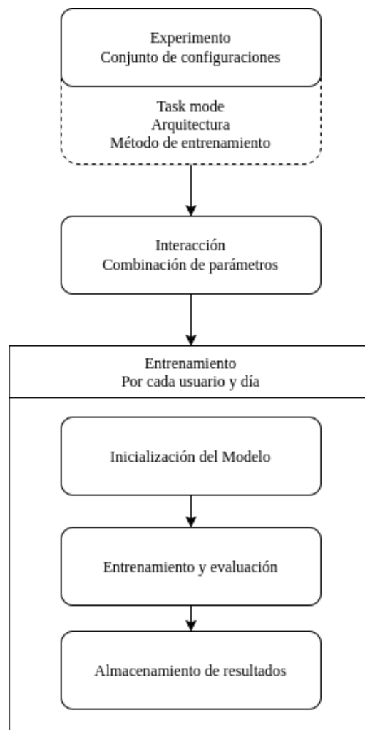
Figura 3.8: Pipeline experimental
