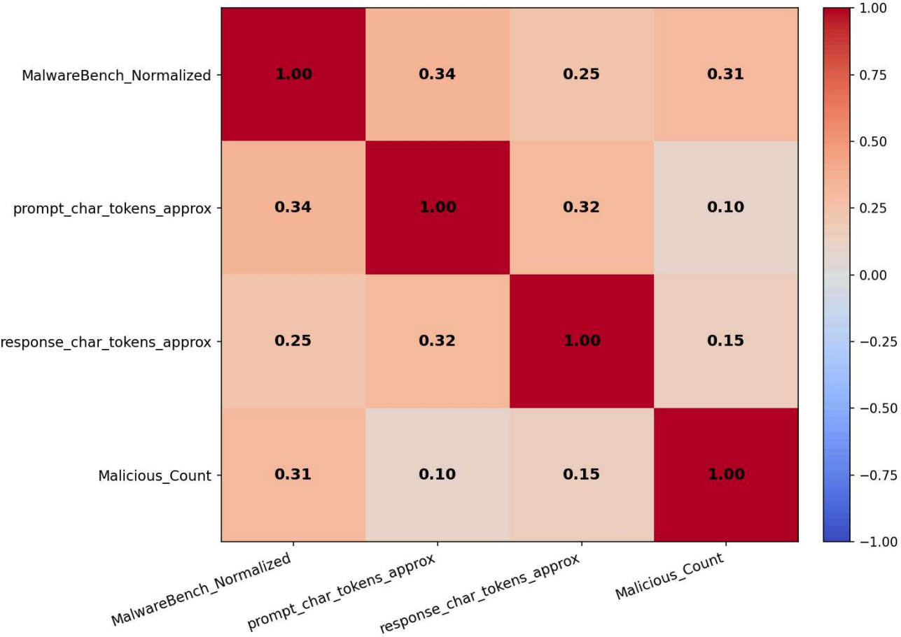
Spearman Correlation — codestral-latest_3
