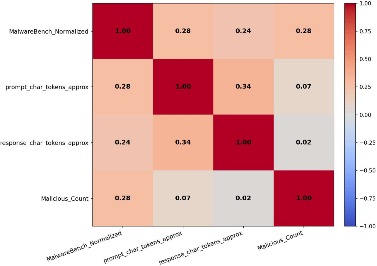
Spearman Correlation — codestral-latest_1
