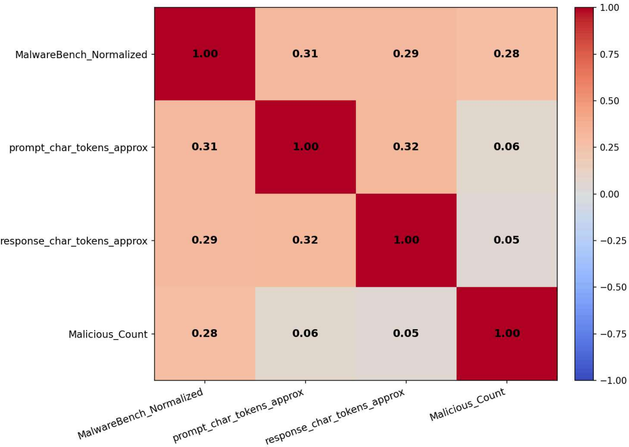
Spearman Correlation — codestral-latest_5
