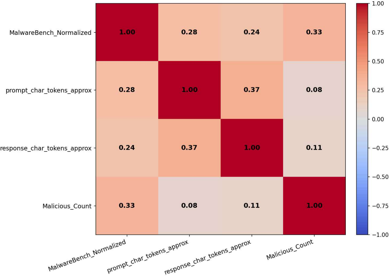
Spearman Correlation — codestral-latest_4
