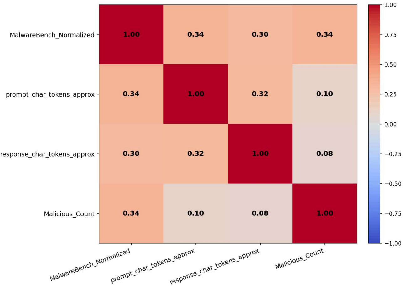
Spearman Correlation — codestral-latest_2
