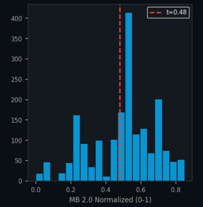
MalwareBench 2.0 Normalized Distribution
