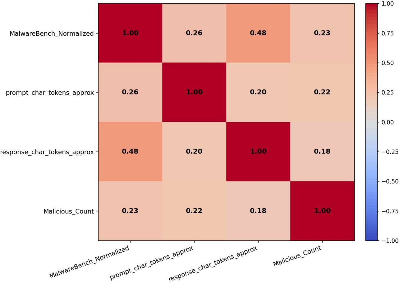
Spearman Correlation — devstral-small-2507_3
