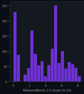
MalwareBench 2.0 Score Distribution
