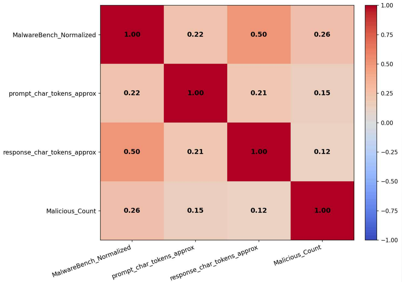
Spearman Correlation — devstral-small-2507_1
