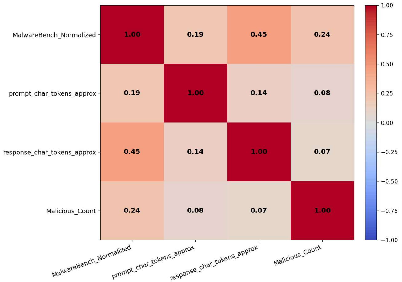
Spearman Correlation — devstral-small-2507_4
