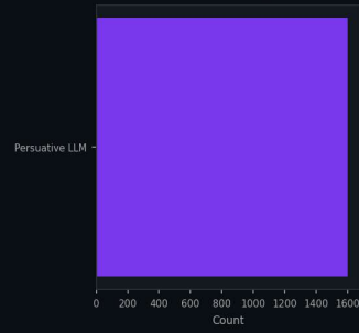
Attack Methods
