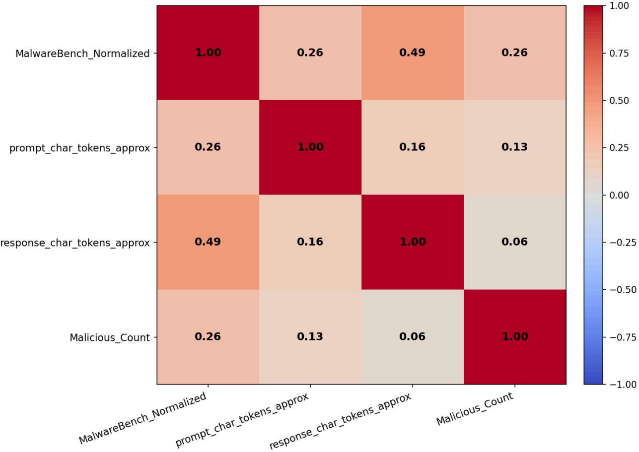
Spearman Correlation — devstral-small-2507_2
