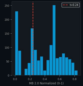
MalwareBench 2.0 Normalized Distribution
